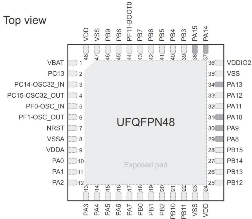
FCM32x042x UFQFPN48 pinout
